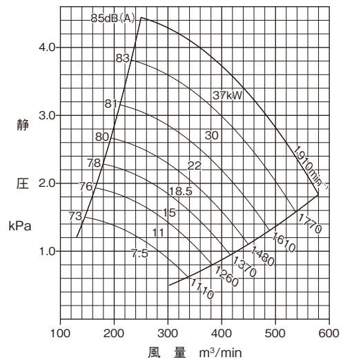
CTF3-No.6½
