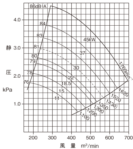
CTF3-No.7
