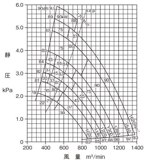
CTF3-No.7
